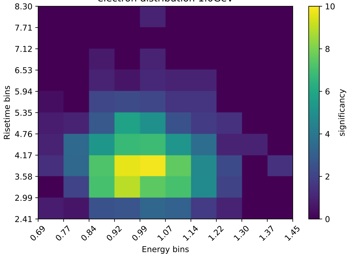
electron distribution 1.0GeV
